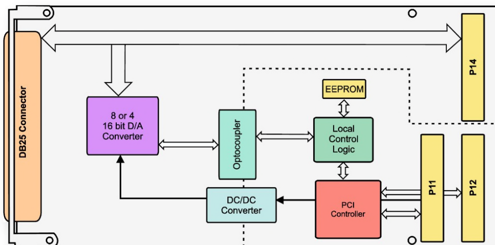
Figure 1-1 : Block Diagram
