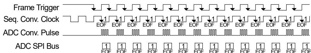
Example: Frame Interval = 1 Conversion Clock, Conversions per Frame= 1
