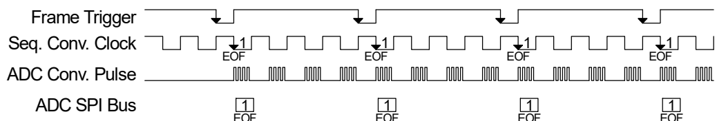
Example: Frame Interval = 4 Conversion Clocks, Conversions per Frame= 1
