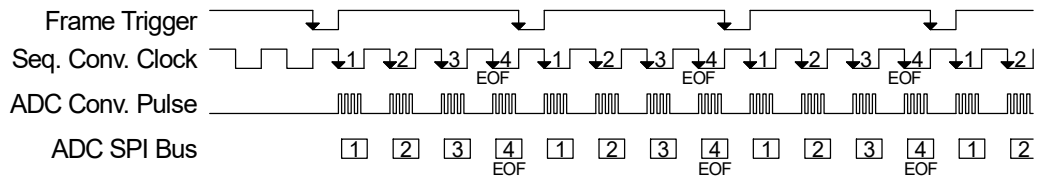
Example: Frame Interval = 4 Conversion Clocks, Conversions per Frame = 4
