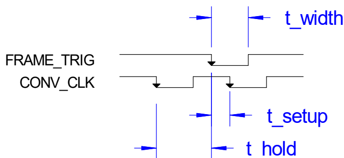
Figure 9-10 : Frame Trigger Timing Requirements
