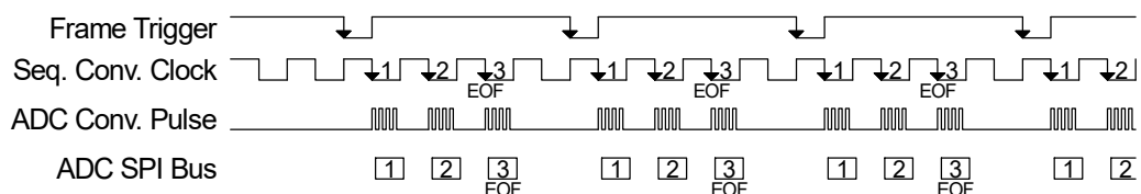
Example: Frame Interval = 4 Conversion Clocks, Conversions per Frame= 3
