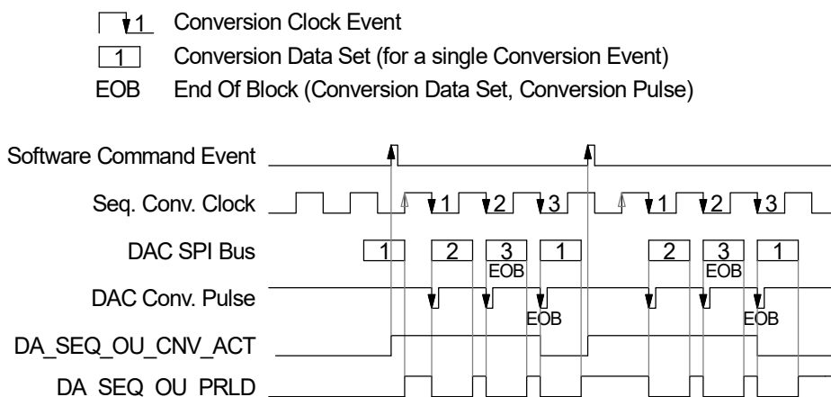
Figure 9-2 : Normal Mode Example Diagram (D/A)
